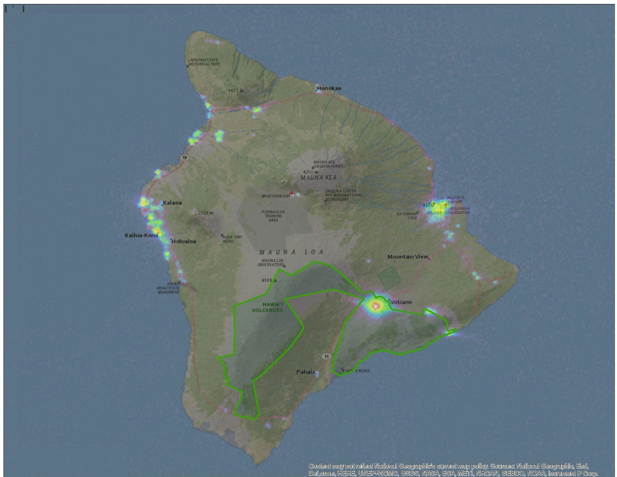
Figure 1. False color VIIRS satellite image of the Island of Hawai'i. The imager is sensitive to green through red light and infrared light, but not to blue light. Lava from Kilauea is bright in this image (with a lot of infrared light), but Kilauea adds very little additional light over Maunakea because the glow from the lava is so red. Major light sources include Hilo, Kona, hotels along
