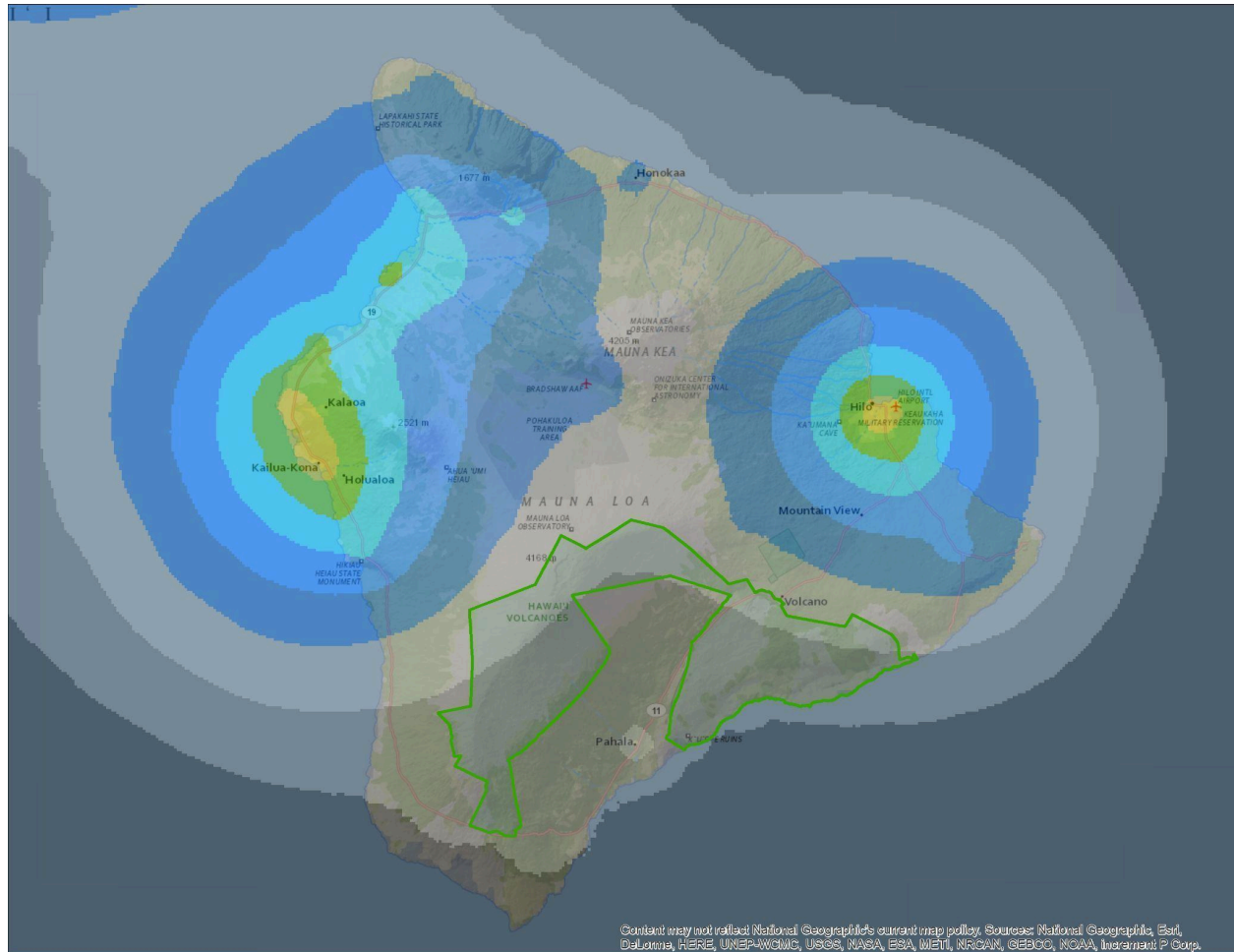
Figure 2. Map of artificial light over the Island of Hawai'i. The contribution from the volcano (natural light) was removed since the lava glow is so red, and the VIIRS image includes infrared light that is not seen by the human eye, and has less scattering. Although not bright, the light from the Pohakuloa Training Area adds significantly to the artificial light over Maunakea due to its proximity (6 miles away).
